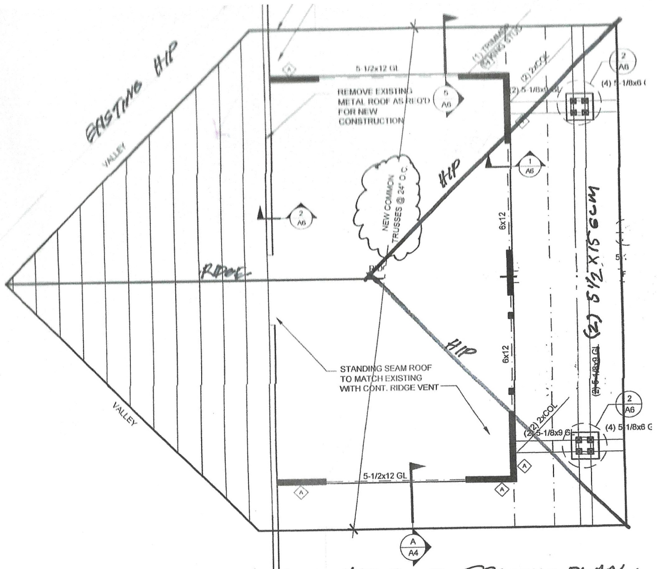
1 ALTERNATE HIP ROOF FRAMING PLAN - FRAMING PLAN @ BUILDING EXPANSION SCALE: 3/16" = 1'-0"
